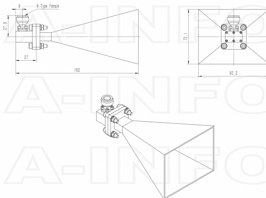
N Type Female Output (P/N: LB-62-20-C-NF)
